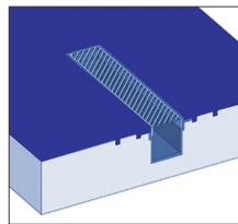
Finished floor showing the filled anchor grooves.
